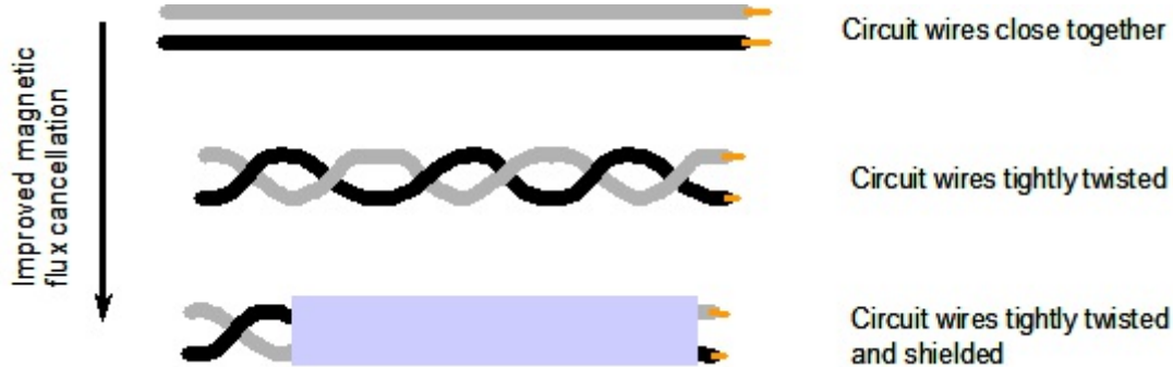
Figure 229.4 Wires of the same circuit arranged close together will achieve good magnetic flux cancellation, by twisting the pair of wires together achieves even better magnetic flux cancellation. Placing a thin metal shield around the pair of twisted wires is an effective way to prevent any remaining magnetic flux from influencing other adjacent wires.
