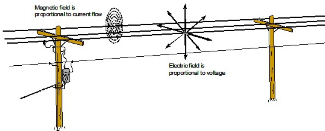
Figure 229.1 An energized wire with a voltage, but no current will produce an electrical field. A wire carrying current with little voltage will produce a magnetic field. A wire with high voltage and high current will produce a strong magnetic field and a strong electric field.
