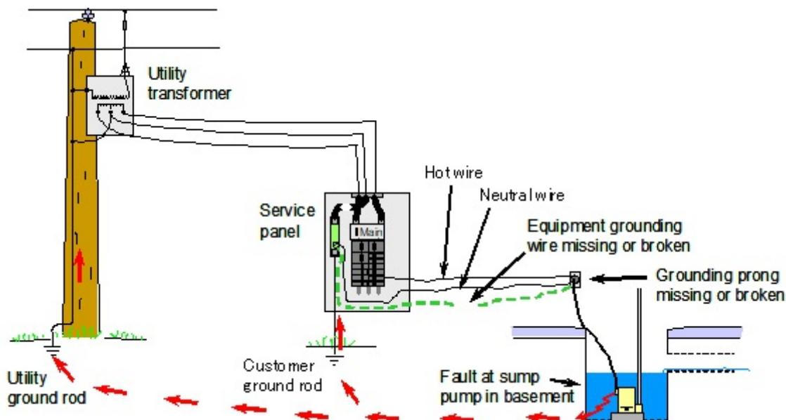
Figure 228.5 A fault in equipment that is not grounded may result in an earth current that can cause an objectionable or even dangerous voltage to occur in the surrounding area.
