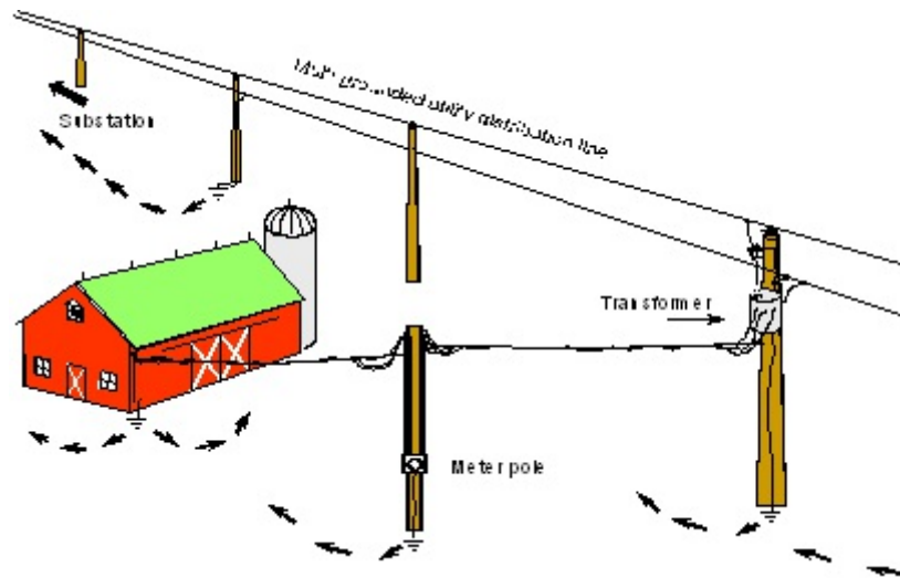
Figure 337.1 The small amount of power line neutral current that flows in the earth returns to the a grounding system at the substation supplying power to the distribution line.
