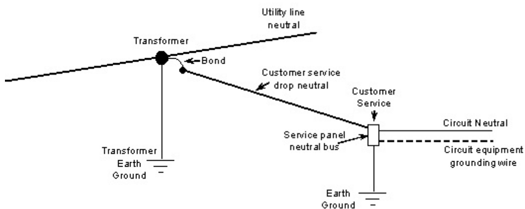
Figure 337.3 In most cases the utility neutral wire is solidly connected to the customer neutral. This illustration only shows system neutrals and grounds.
