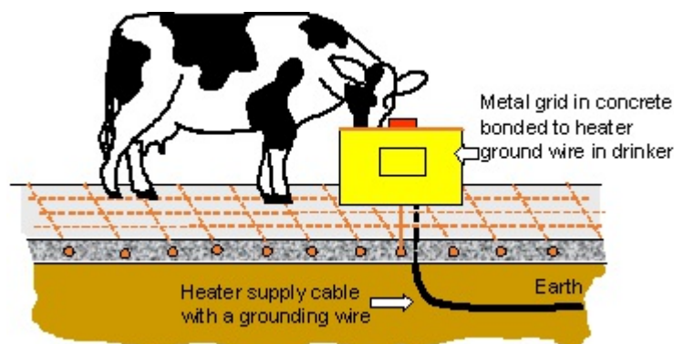
Figure 337.11 Equipotential planes are required by code in areas where livestock are likely to become a part of an NEV path to earth.
