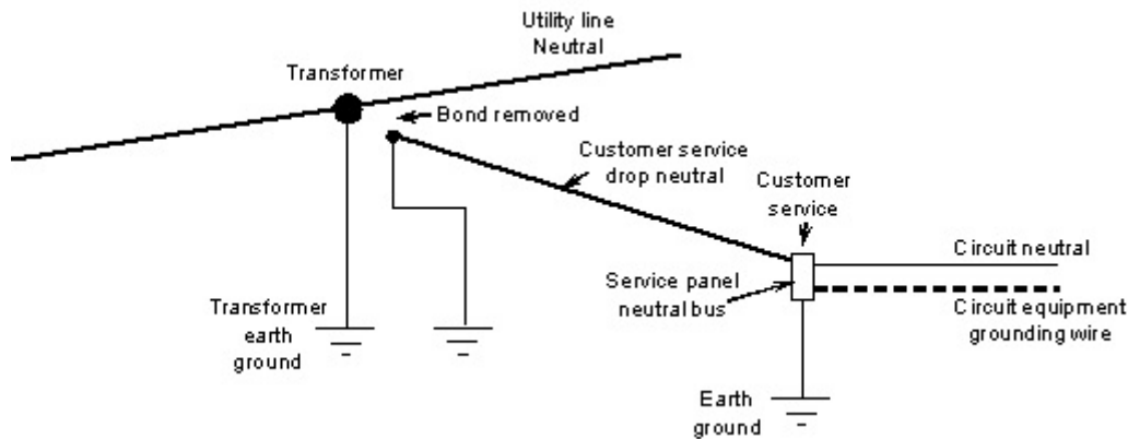
Figure 337.4 Off property NEV sources can be prevented from accessing a customer electrical system by removing the primary/secondary bond at the transformer. In the rare case when the primary/secondary neutral bond is removed at a transformer, a second ground must be added to the customer side neutral at the transformer.
