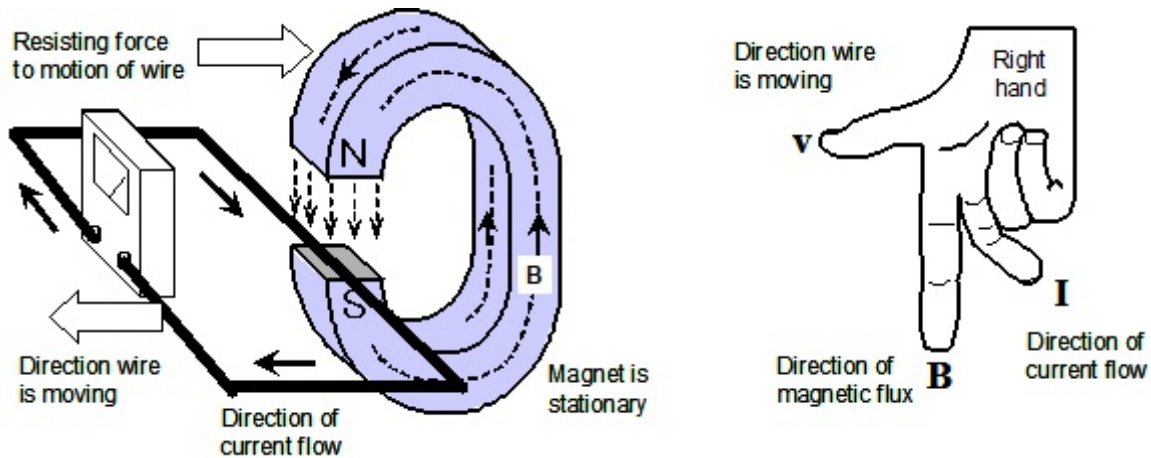
Figure 217.8 If a wire forming a circuit is moved through a magnetic flux, a current will flow in the wire. The right hand rule can be used to determine the direction of current flow in the wire knowing the direction of magnetic flux and direction the wire is moving with respect to the magnetic flux.
