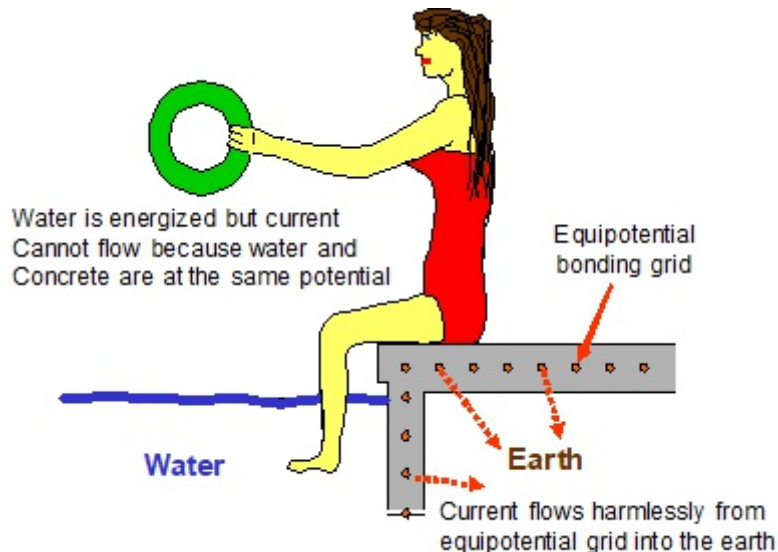
Figure 338.4. An equipotential grid should be installed in walkways around the pool and extending out from the edge of the pool at least 3 feet.
