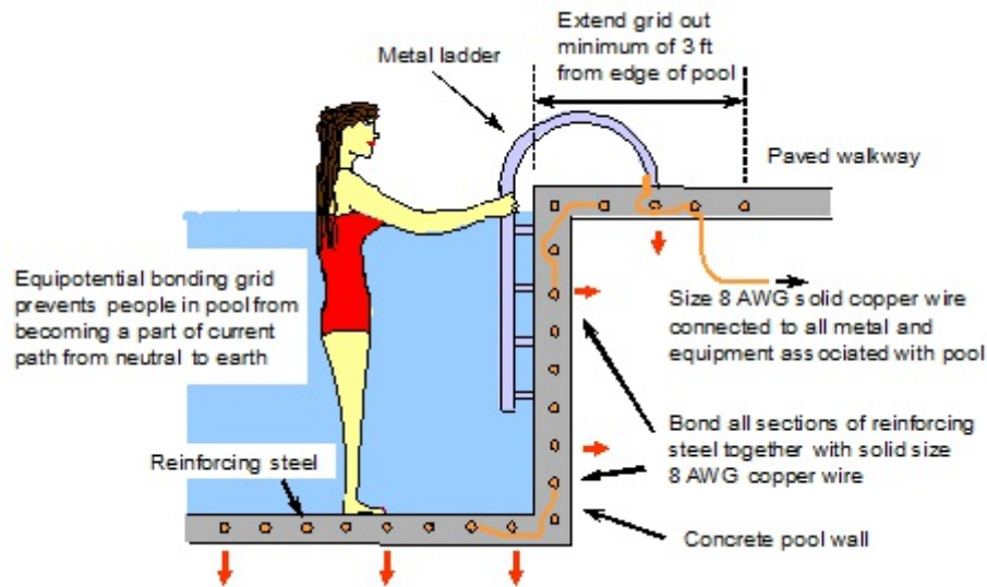
Figure 338.3 Metal steel reinforcing installed in swimming pool concrete walls and floor forms an equipotential grid that prevents a person in the pool from becoming part of a neutral-to-earth voltage circuit.
