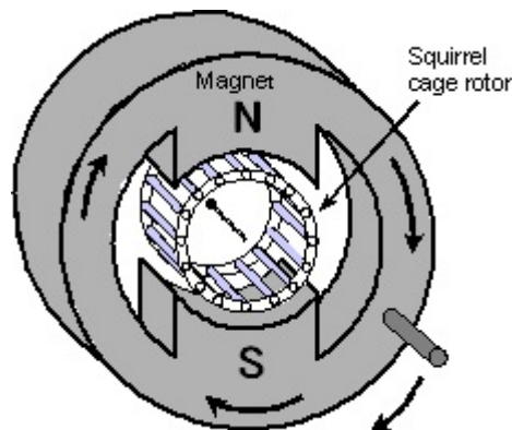
Figure 312.1 The basic parts of an induction motor are a metal cylinder resembling a squirrel cage mounted on a turning shaft and surrounded by a stator with a rotating magnetic field.
