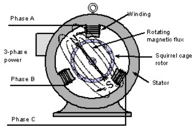
Figure 312.2 A rotating magnetic flux can be achieved by placing three windings on a steel core (stator) and energizing the windings with 3-phase power.
