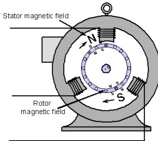
Figure 312.4 This end view of an induction motor shows the magnetic poles created by the induced current flow in the squirrel cage rotor with respect to the stator rotating magnetic flux.
