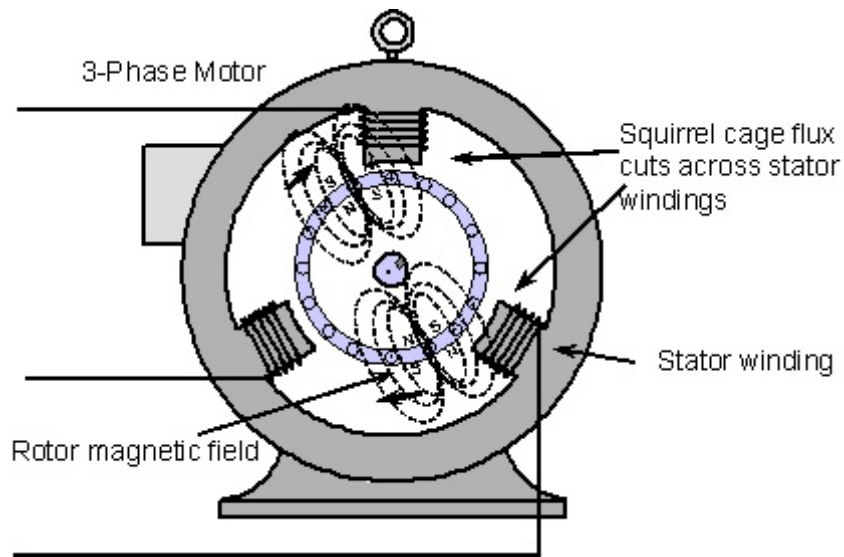
Figure 312.6 The induced current in the squirrel cage of the rotor produces a rotor magnetic field that cuts across the stator windings as the rotor turns and induces a reverse voltage into the stator windings that limits current drawn by the motor.
