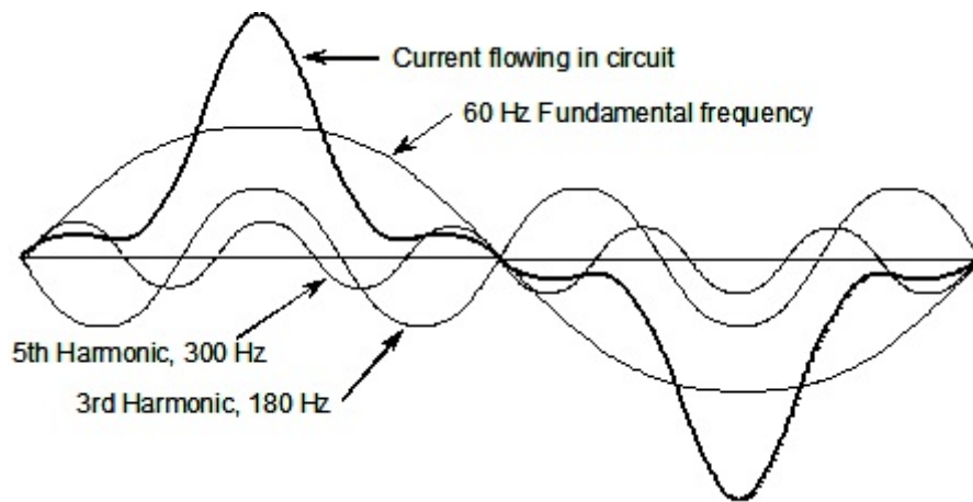
Figure 231.6 The equipment supplied by this circuit causes 3rd and 5th harmonic currents to flow which combine with the 60 Hz current to create an alternating current wave with a high central peak.
