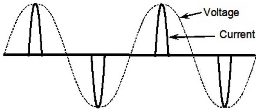
Figure 231.4 A computer draws current in pulses. Even though the voltage supplying the current is nearly a sine wave, the current flow to the computer is not a sine wave. A true rms ammeter is required to accurately measure the current draw of a computer and most electronic equipment.
