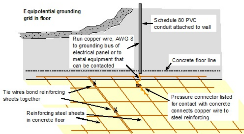
Figure 228.7 A typical means of establishing an equipotential grid is to insure that reinforcing bars or wire mats installed in concrete floors are connected together and a wire brought out of the concrete for connection to exposed metal equipment or electrical supply panel grounding.
