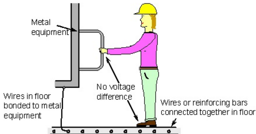
Figure 228.4 Reinforcing metal installed in a concrete floor and bonded to exposed metal above will result in an equipotential bonding grid where there is little or no difference in voltage between the floor and the exposed equipment.
