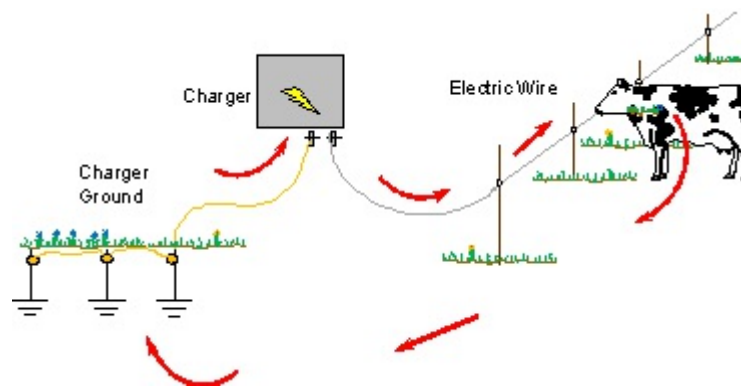
Figure 337.9 A properly installed fence charger system never used electrical system grounds.
