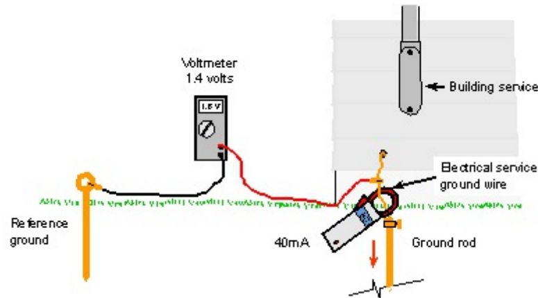
Figure 337.10 Ground rod resistance can often be calculated by measuring the NEV and the current flowing to earth then divide the voltage by the current in amperes.
