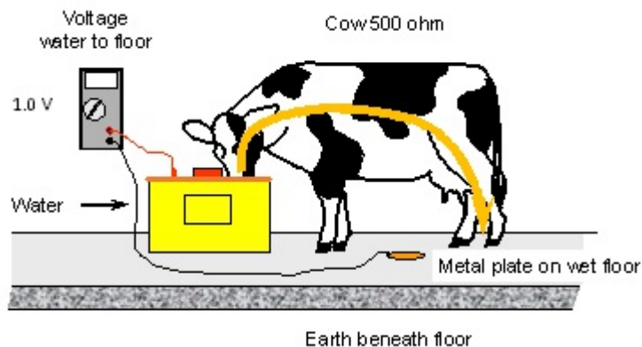
Figure 337.2 This animal can feel current when it is drinking due to a level of neutral-to-earth voltage that can be measured between the water drinker and the wet concrete where the animal is standing.
