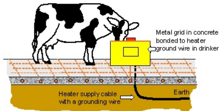
Figure 337.11 Equipotential planes are required by code in areas where livestock are likely to become a part of an NEV path to earth.
