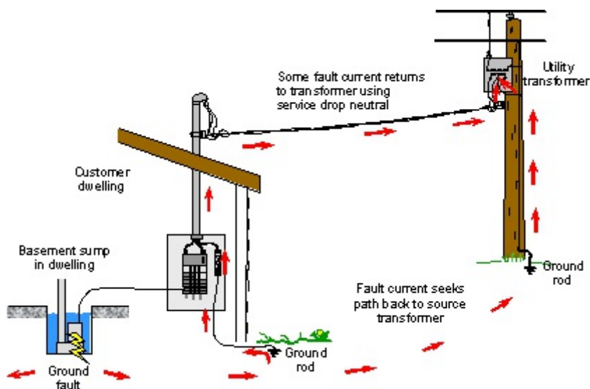
Figure 337.7 Faulting equipment such as this basement sump pump will create NEV as current returns to the utility transformer.
