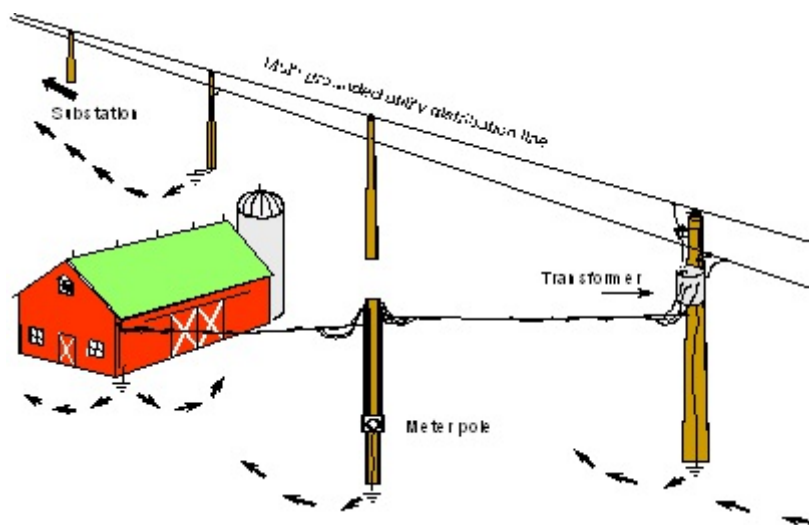
Figure 337.1 The small amount of power line neutral current that flows in the earth returns to the grounding system at the substation supplying power to the distribution line.
