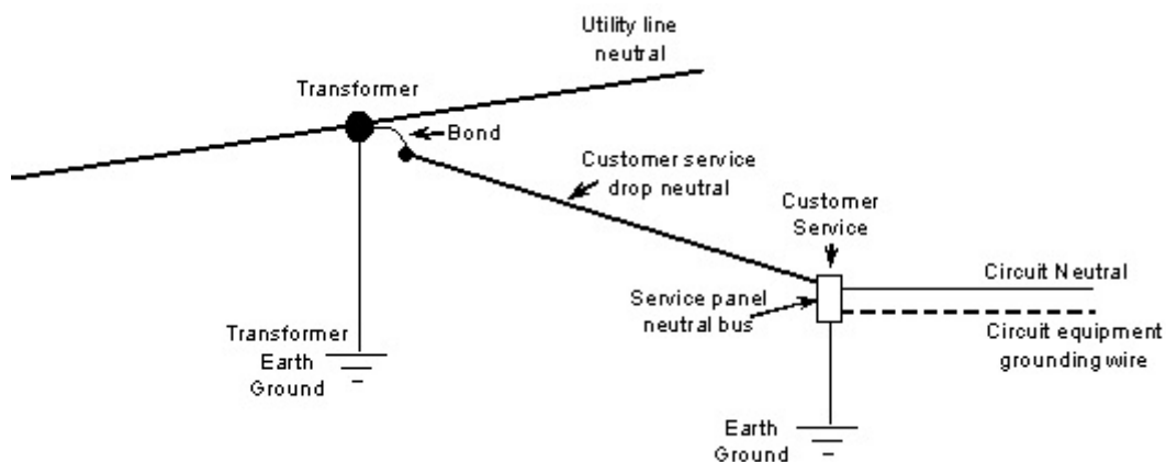
Figure 337.3 In most cases the utility neutral wire is solidly connected to the customer neutral. This illustration only shows system neutrals and grounds.
