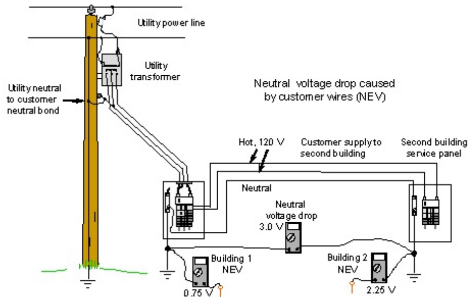
Figure 337.6 Excessive voltage drop on the neutral wire of a feeder line to a remote building can result in neutral-to-earth voltage that is high enough to have an effect on livestock.
