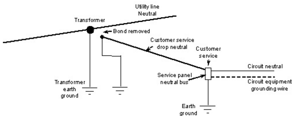
Figure 337.4 Off property NEV sources can be prevented from accessing a customer electrical system by removing the primary/secondary bond at the transformer. In the rare case when the primary/secondary neutral bond is removed at a transformer, a second ground must be added to the customer side neutral at the transformer.
