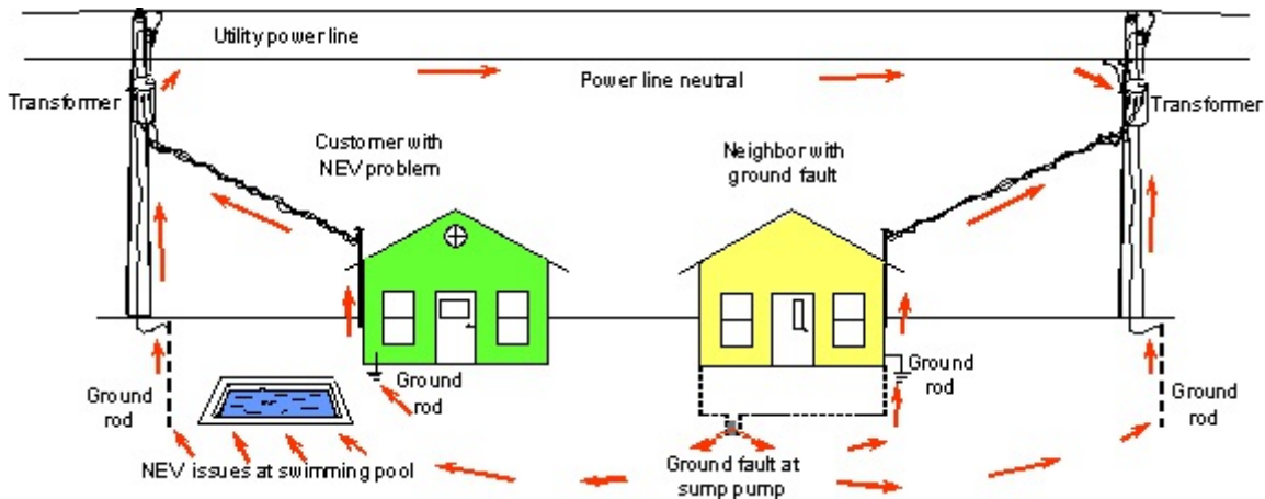
Figure 337.8 The fault current entering the earth at the neighbor's property can travel to all the surrounding neighbor's property to find a path back to the source transformer.
