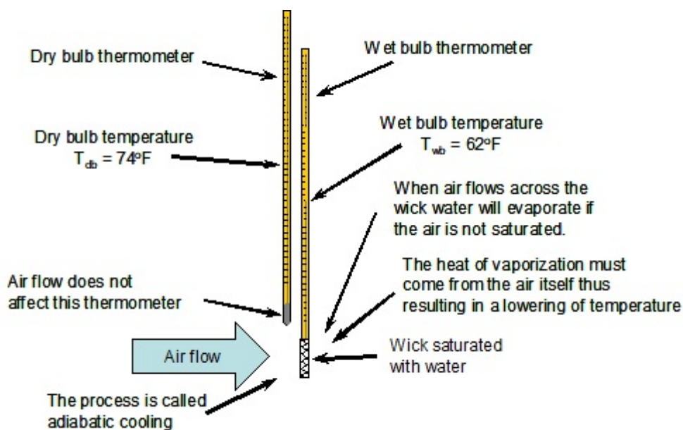
Figure 386.1 A device called a psychrometer, in this case using two thermometers, measures the dry bulb temperature and the wet bulb temperature. With these two measurements the characteristics of air can be determined.
