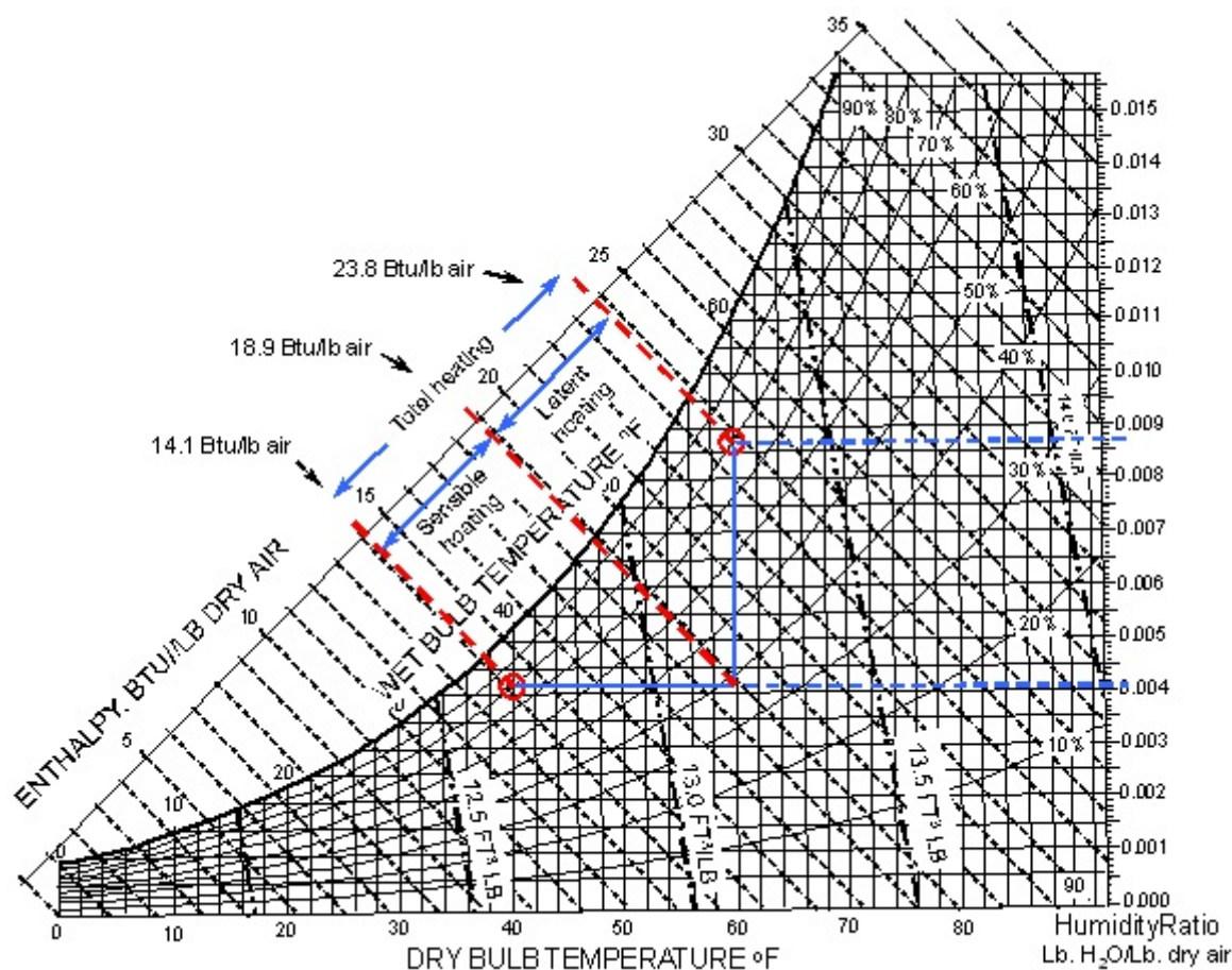
Figure 386.4 The total heat content of the air leaving a confined space as compared to the air entering the confined space can be subdivided into sensible heat change resulting in a temperature change with no change in water content, and a latent heat change which results in a change in water content at a constant temperature.
