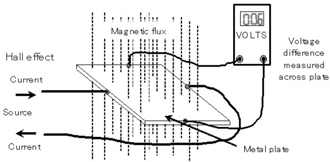
Figure 560.5 If current is passed through a flat metal plate placed in a magnetic flux, a voltage will develop from one side of the plate to the other in proportion to the density of the magnetic flux. This is called the Hall effect.
