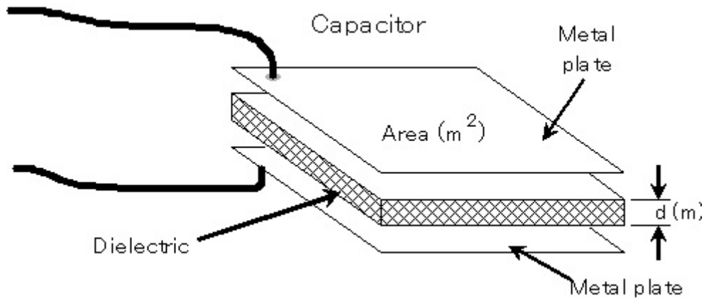
Figure 560.1 A capacitor consists of two metal plates separated by an insulator called a dielectric. When connected to an electrical source, current flows until the dielectric is fully charged and the voltage between the plates equals the voltage of the source.
