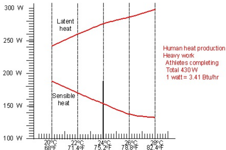
Figure 384.11 Sensible heat and latent heat production for adult human involved in heavy physical work or an athlete involved in vigorous activity. Total heat is the sum of latent and sensible heat.
