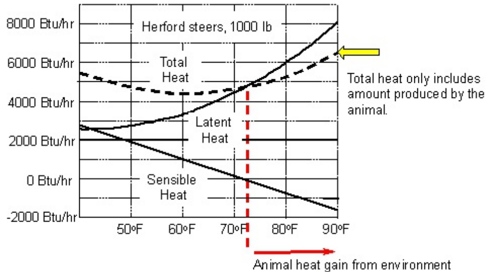
Figure 384.5 Heat production rates for Herford beef cattle.
