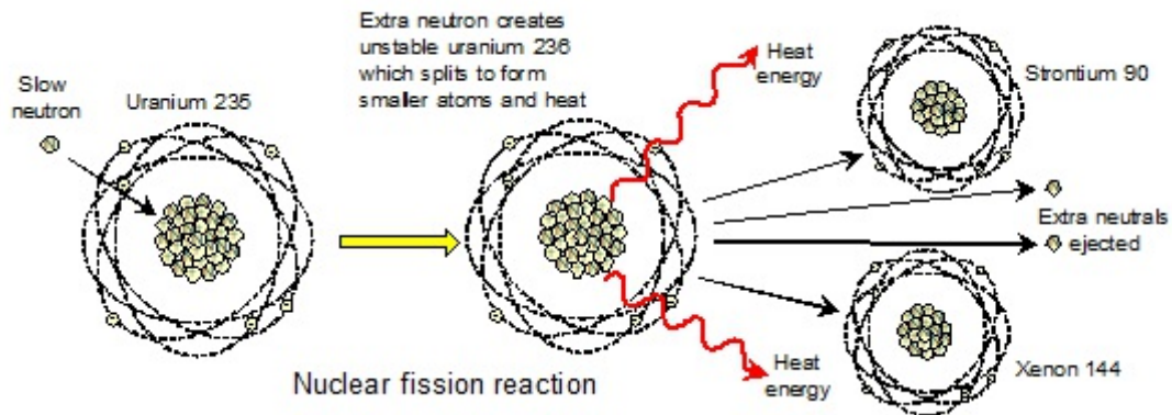
Figure 224.9 A typical fission reaction of uranium U_{235} results in the production of strontium 90 and xenon 144, with the release on one or three neutrons and a lot of energy as heat.
